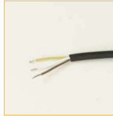
Black Round Cable 3PIN Wire gauge: 0.519mm 2 /20AWG MOQ: 100M/Roll
