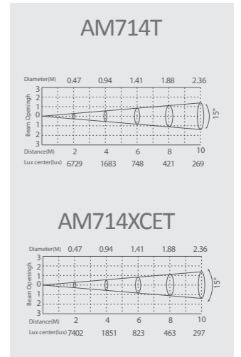
Illuminance diagram
