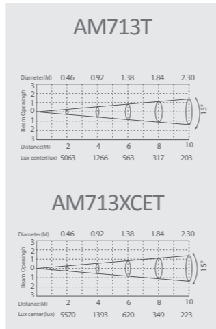
Illuminance diagram
